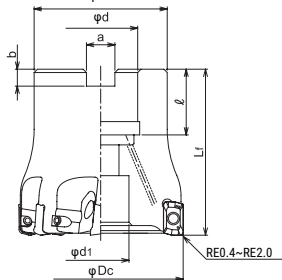
● Shoulder milling
