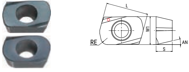
Shoulder insert
